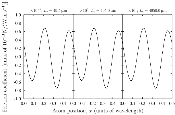
Fig. 6. Spatial dependence of the friction force acting on an atom outside a cavity, with detuning 10\Gamma to the red of resonance. Three different cavity lengths are shown; the friction force scales almost linearly with the cavity length. Note the different scaling factors and cavity lengths, given above each curve. (Parameters as in Sect. 2.3 but with \partial\zeta/\partial k = 0 .)
